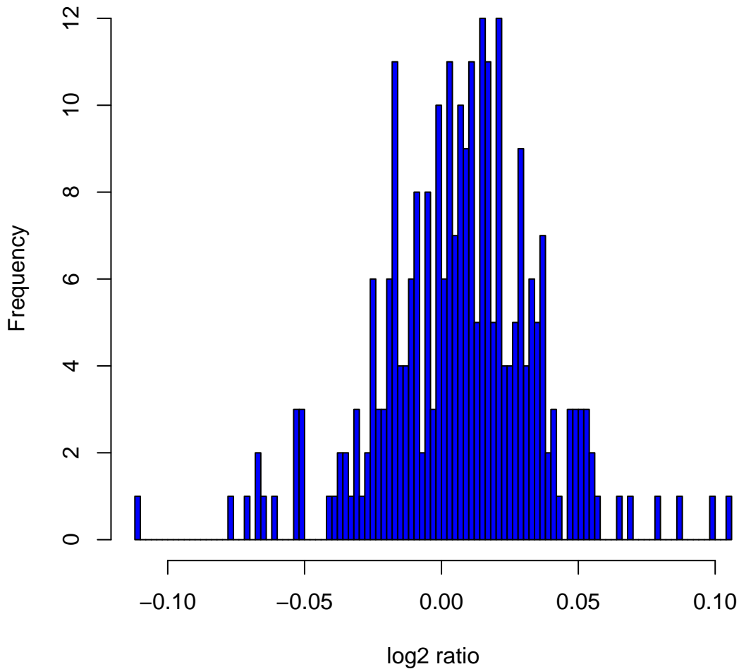
Histogram of log 2 ratios in 270 HapMap samples at clone Chr11tp-4G1
