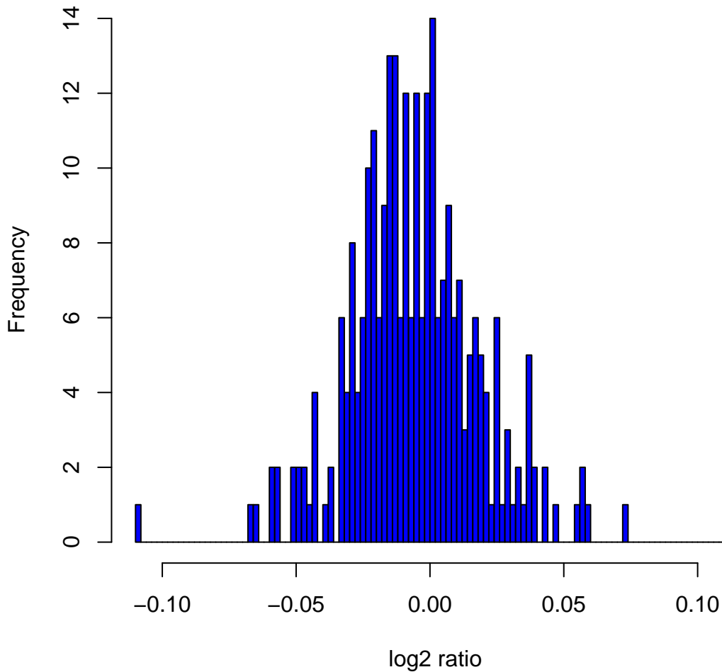
Histogram of \log_2 ratios in 270 HapMap samples at clone Chr11tp-4G5
