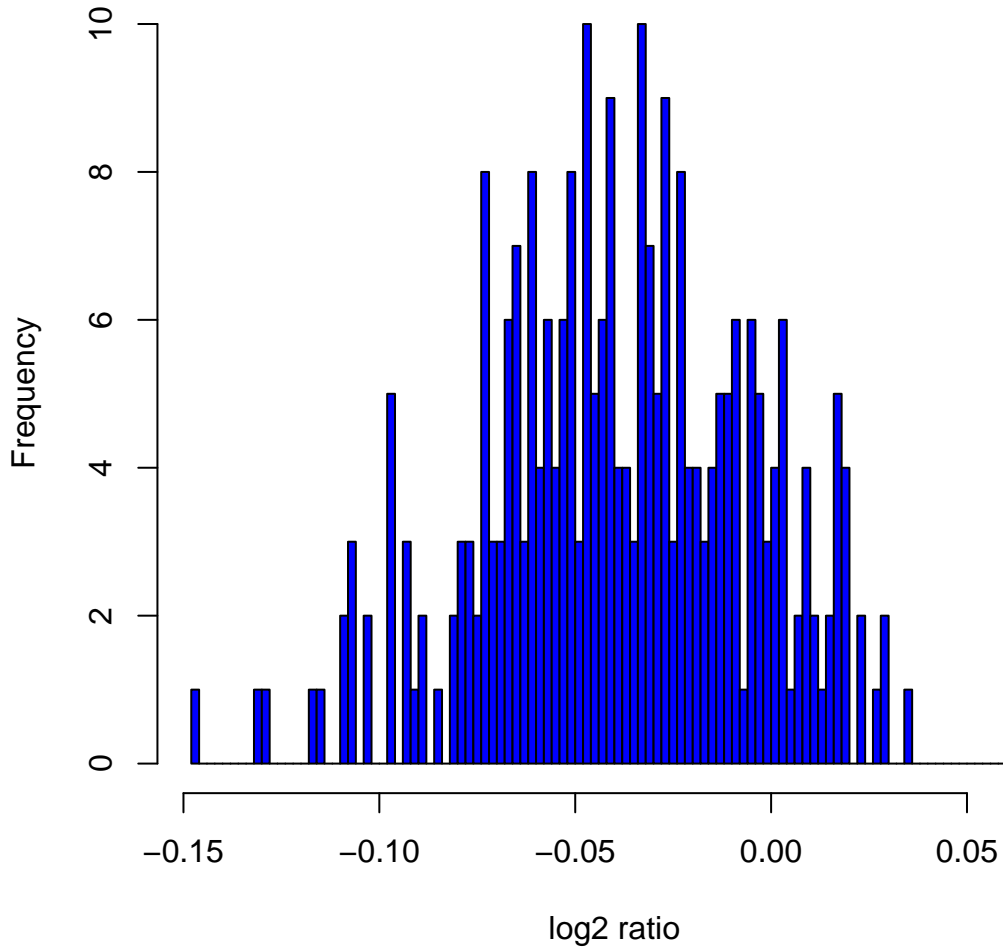
Histogram of \log_2 ratios in 270 HapMap samples at clone Chr11tp-4G7
