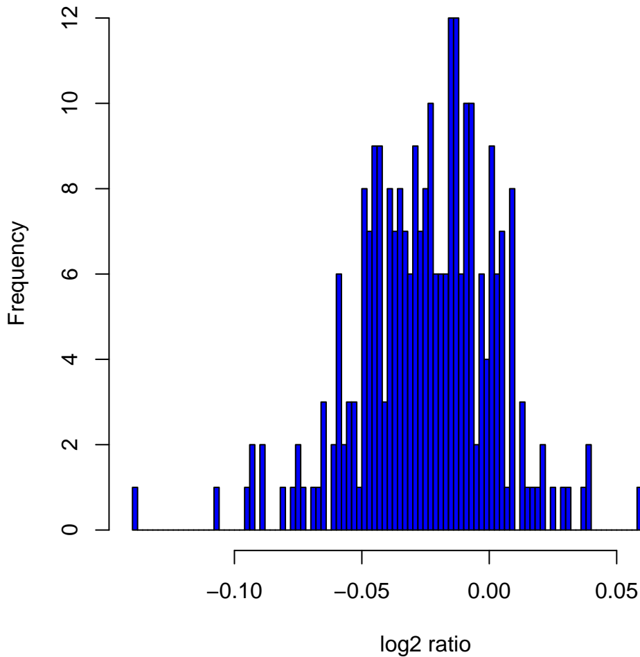
Histogram of log 2 ratios in 270 HapMap samples at clone Chr11tp-4G8
