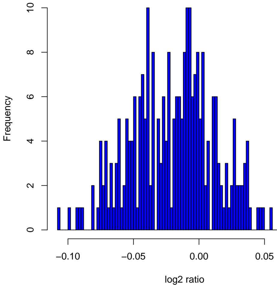
Histogram of log 2 ratios in 270 HapMap samples at clone Chr11tp-4H8
