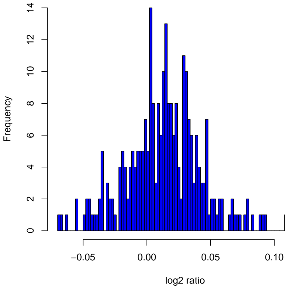
Histogram of log2ratios in 270 HapMap samples at clone Chr11tp-5A10
