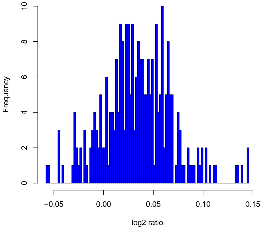
Histogram of \log_2 ratios in 270 HapMap samples at clone Chr11tp-5C2
