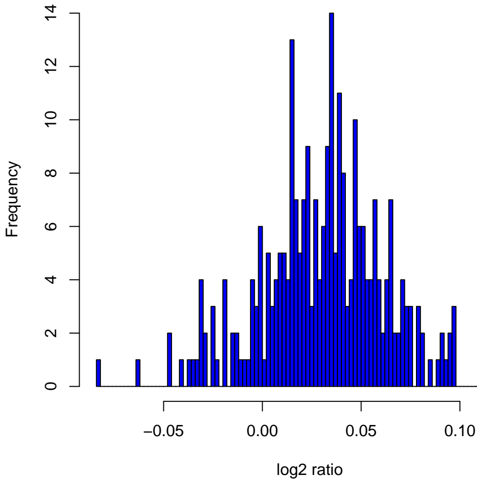
Histogram of log2ratios in 270 HapMap samples at clone Chr11tp-5D12
