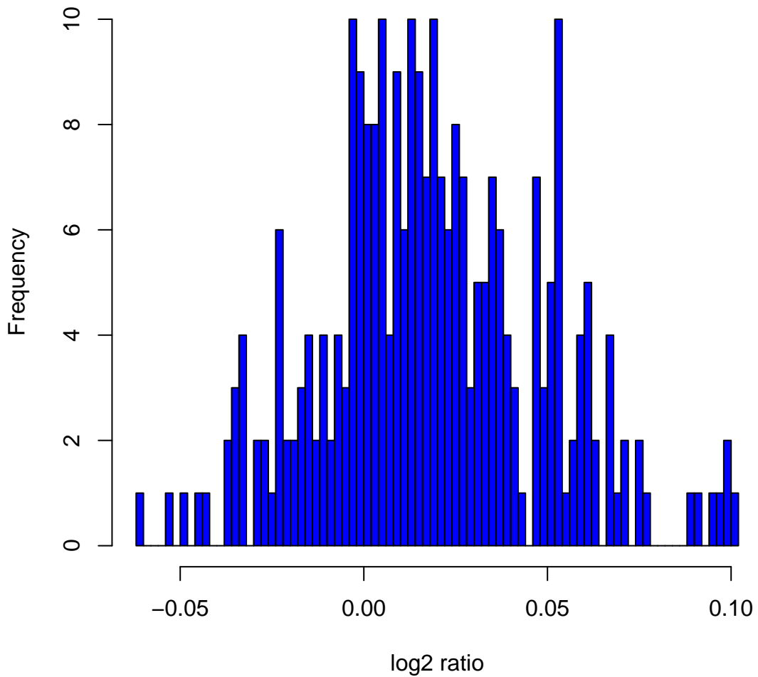
Histogram of log 2 ratios in 270 HapMap samples at clone Chr11tp-5D3
