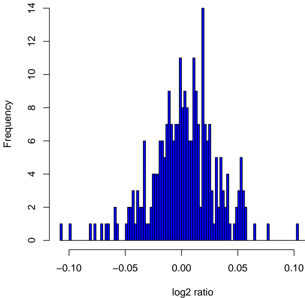
Histogram of log 2 ratios in 270 HapMap samples at clone Chr11tp-5E6
