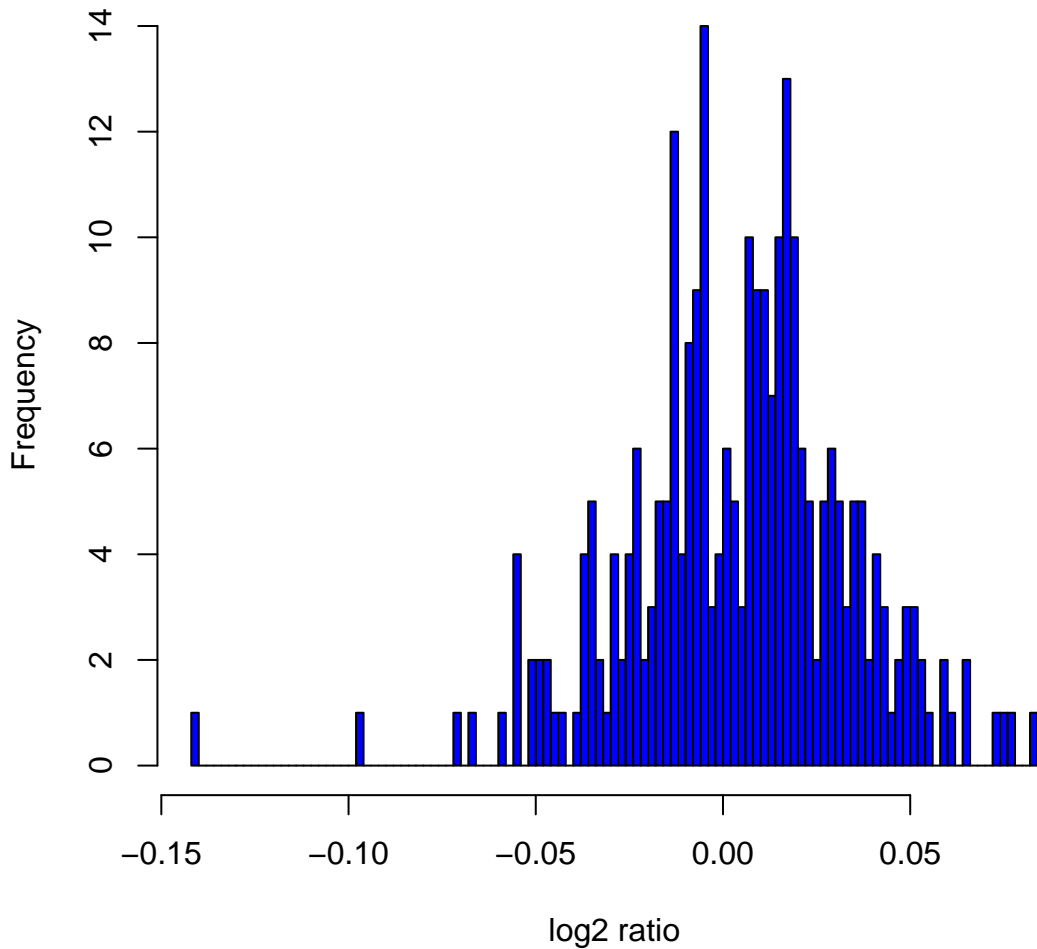
Histogram of log2ratios in 270 HapMap samples at clone Chr11tp-7B12
