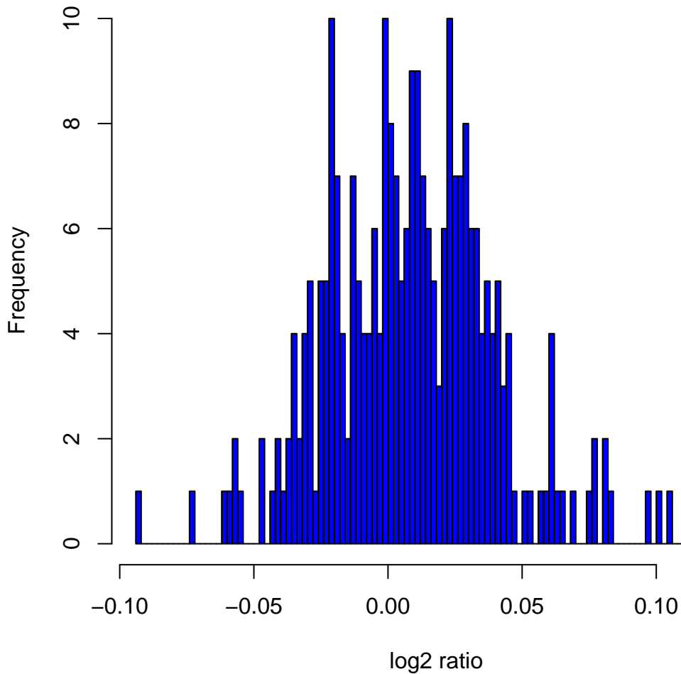
Histogram of \log_2 ratios in 270 HapMap samples at clone Chr11tp-7C1
