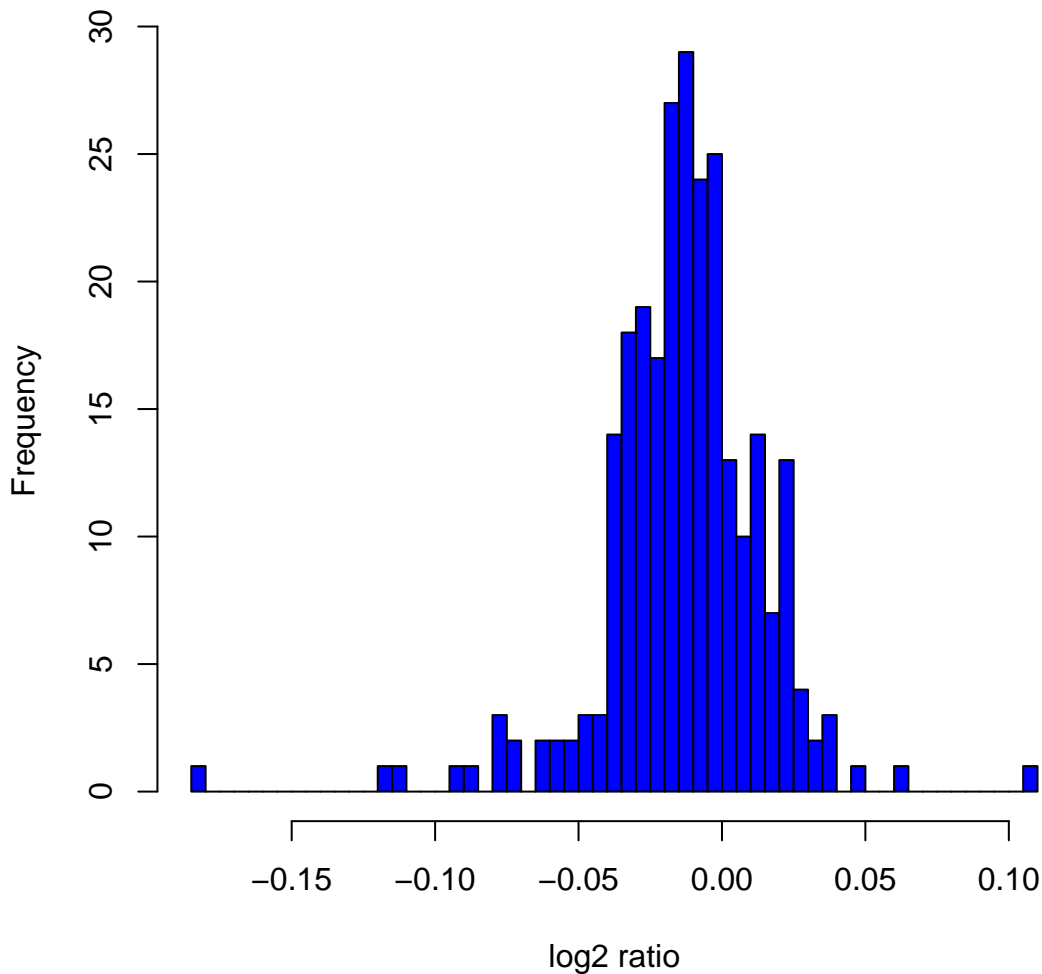
Histogram of log2ratios in 270 HapMap samples at clone Chr11tp-7C11
