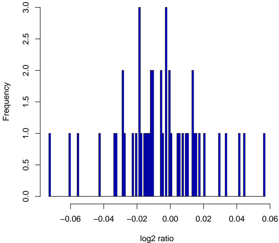
Histogram of log2ratios in 270 HapMap samples at clone Chr11tp-7F11
