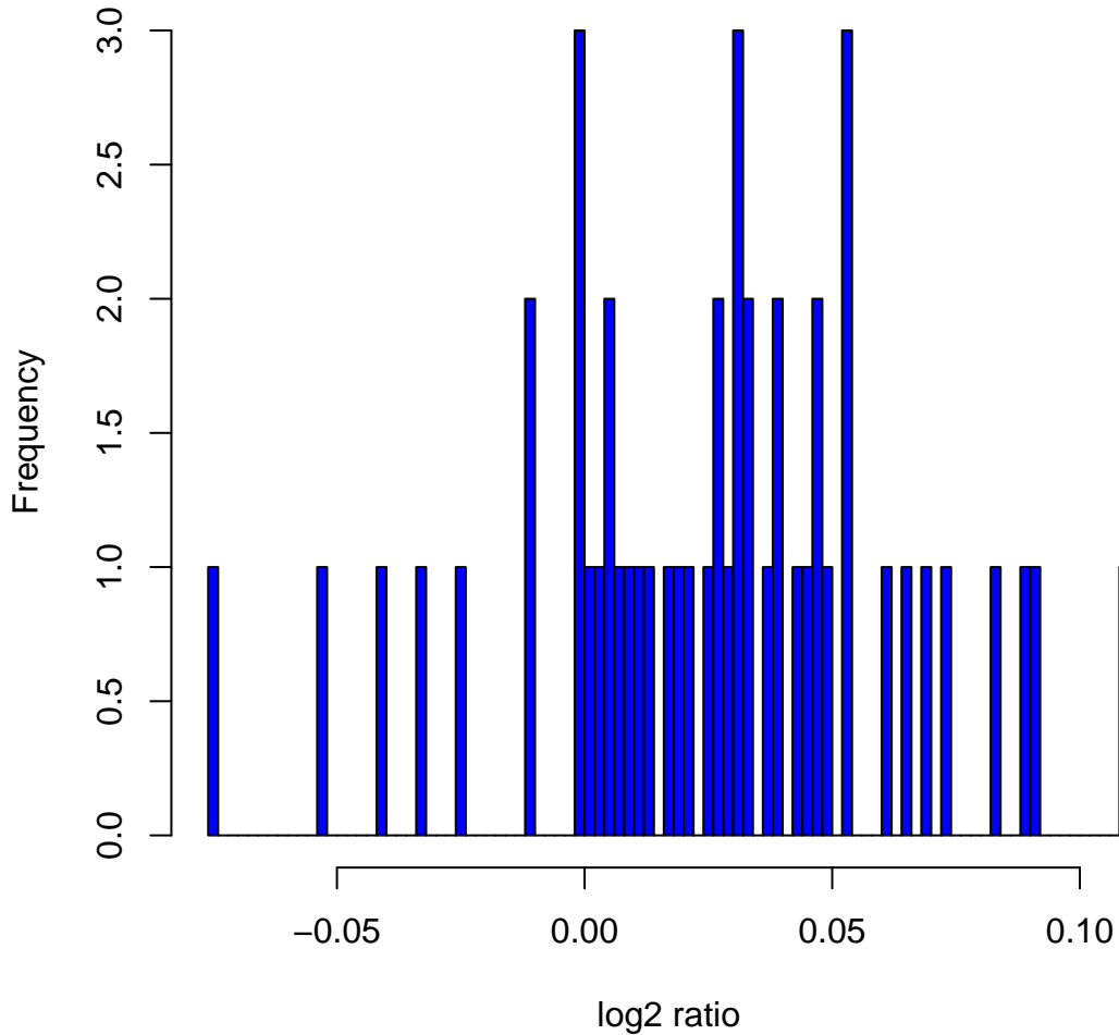
Histogram of log 2 ratios in 270 HapMap samples at clone Chr11tp-7F2
