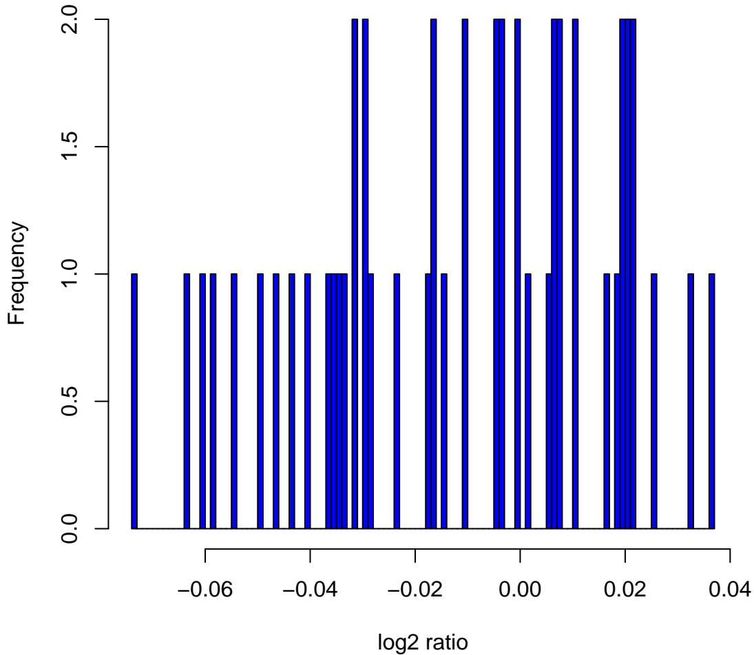
Histogram of log2ratios in 270 HapMap samples at clone Chr11tp-7F4
