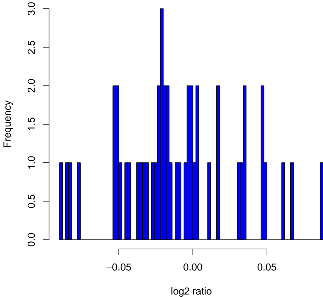
Histogram of log 2 ratios in 270 HapMap samples at clone Chr11tp-7F8
