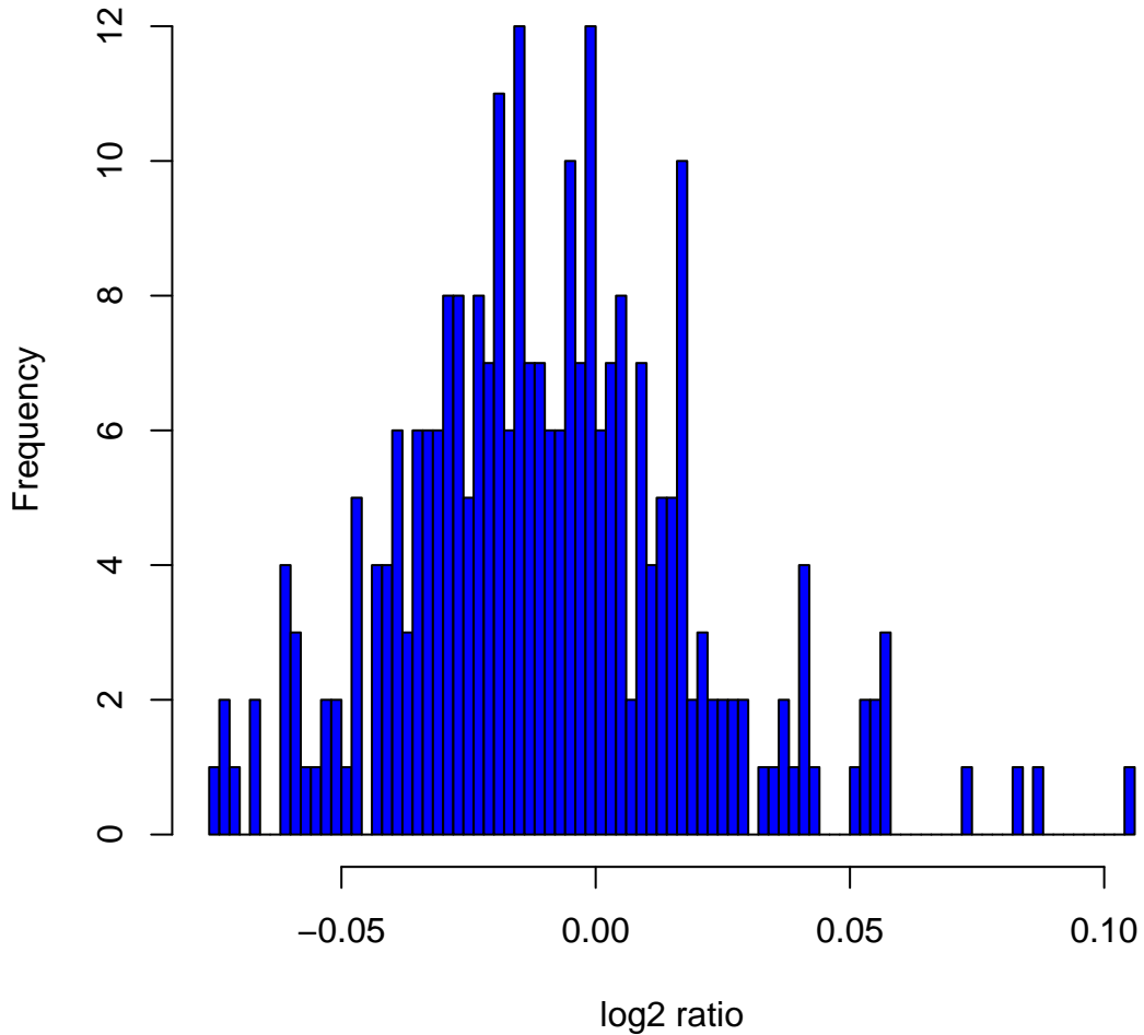
Histogram of \log_2 ratios in 270 HapMap samples at clone Chr11tp-7G3
