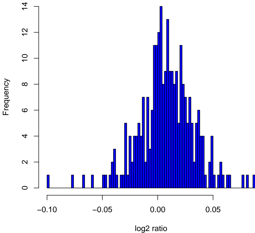
Histogram of log2ratios in 270 HapMap samples at clone Chr11tp-8A11
