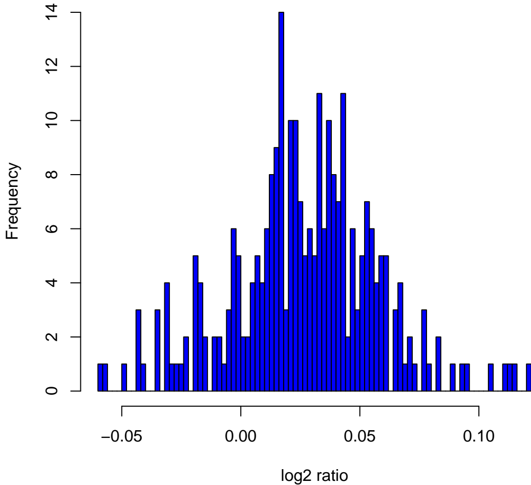
Histogram of log 2 ratios in 270 HapMap samples at clone Chr11tp-8A8
