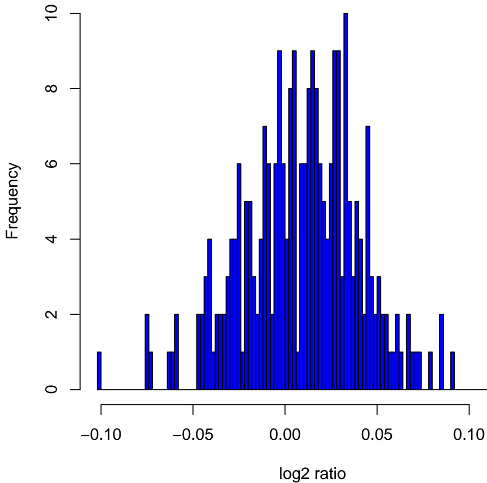
Histogram of log2ratios in 270 HapMap samples at clone Chr11tp-8B10
