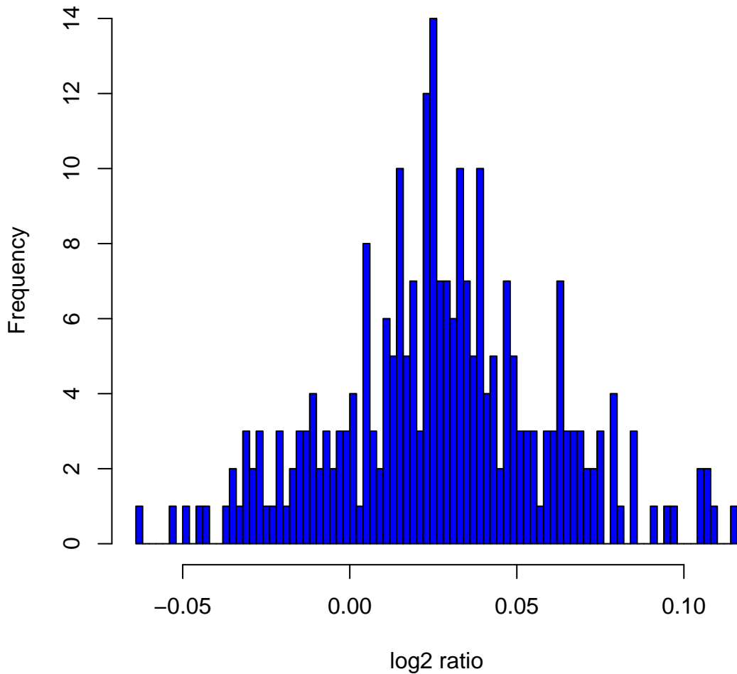
Histogram of log 2 ratios in 270 HapMap samples at clone Chr11tp-8B7
