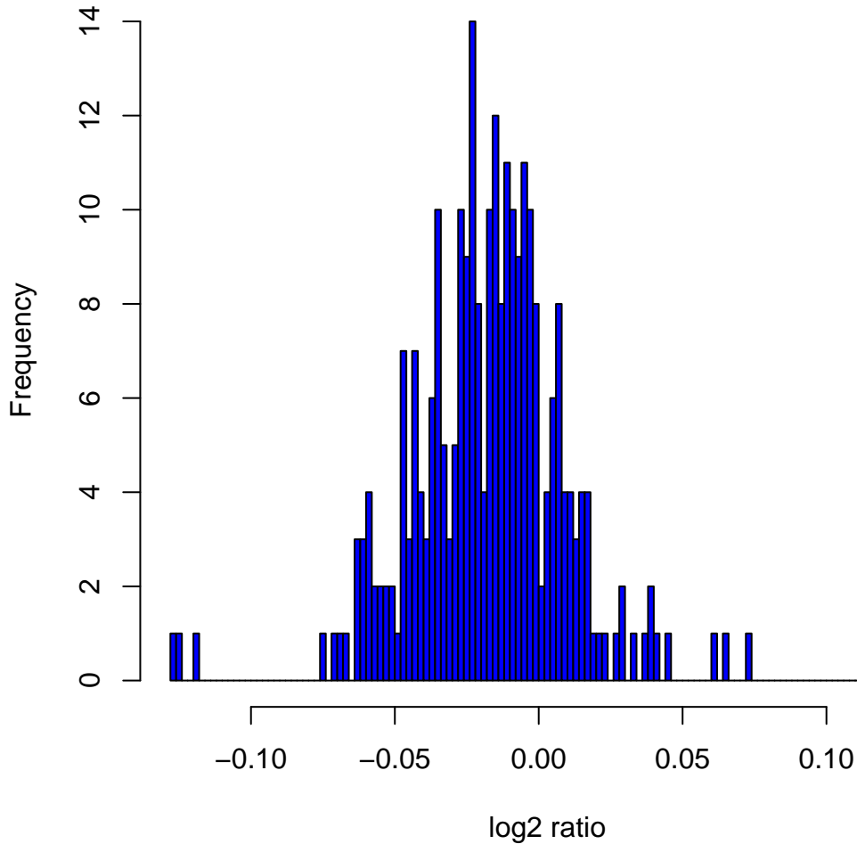
Histogram of log 2 ratios in 270 HapMap samples at clone Chr11tp-8G7
