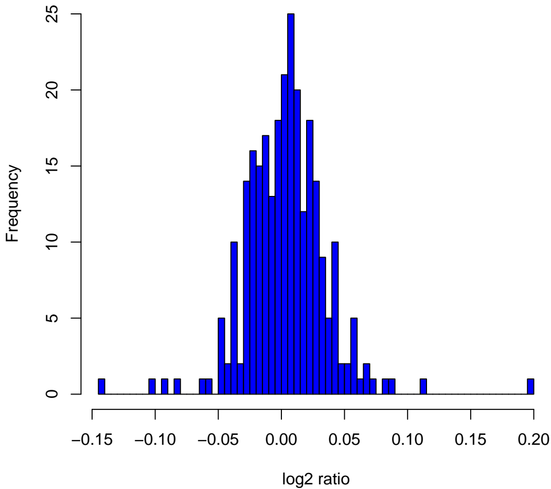
Histogram of log2ratios in 270 HapMap samples at clone Chr11tp-9A4
