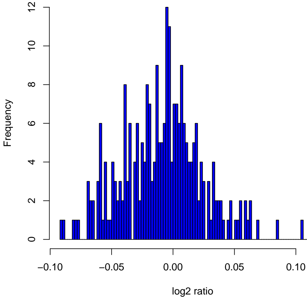
Histogram of log2ratios in 270 HapMap samples at clone Chr11tp-9C11
