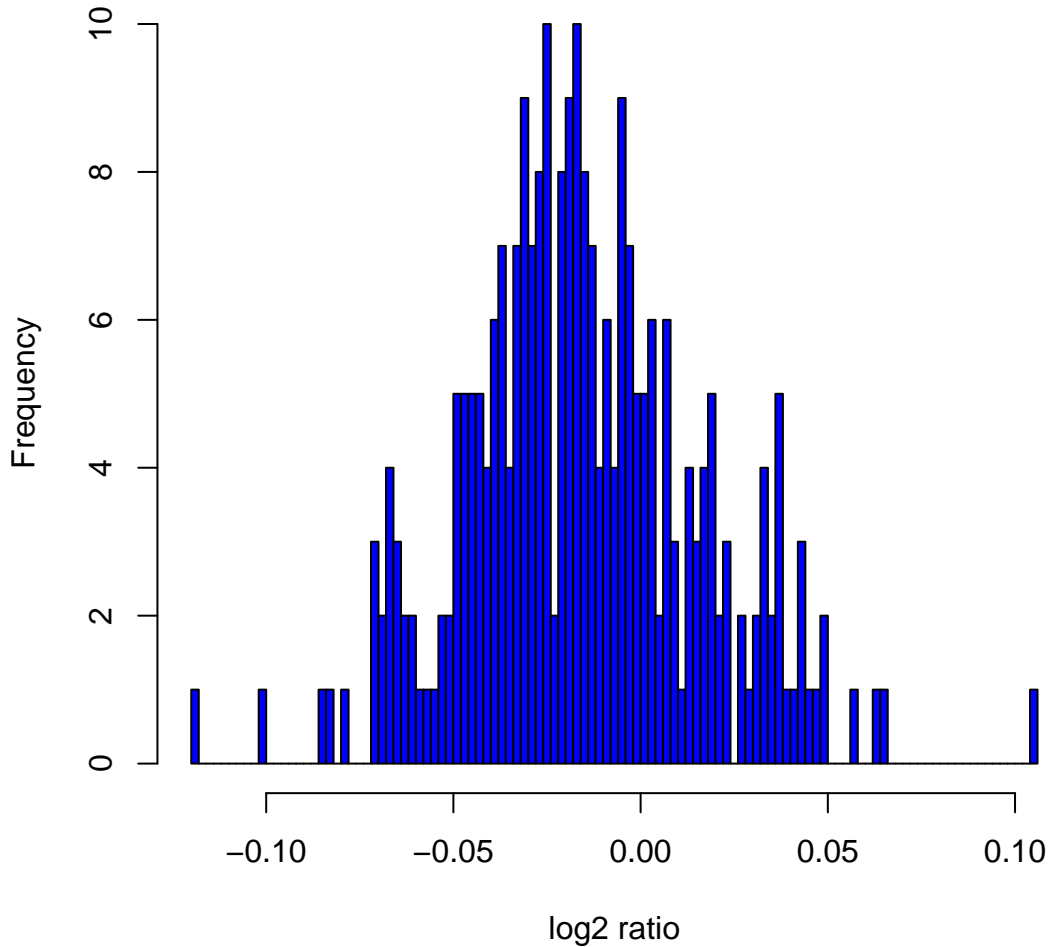
Histogram of log2ratios in 270 HapMap samples at clone Chr11tp-9D11
