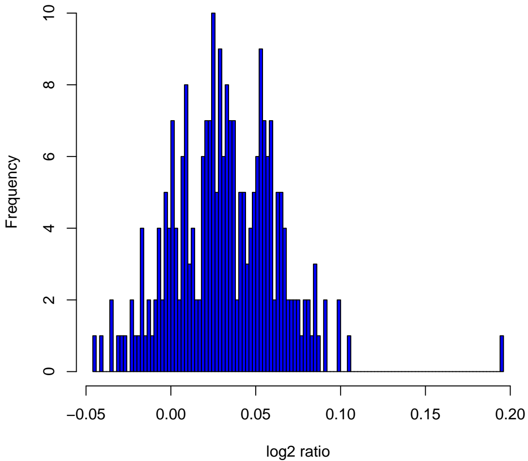
Histogram of log 2 ratios in 270 HapMap samples at clone Chr11tp-9E5
