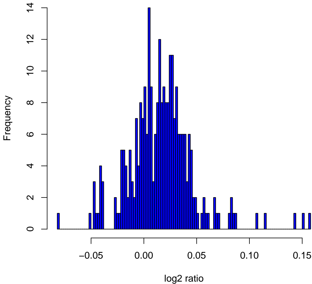
Histogram of log 2 ratios in 270 HapMap samples at clone Chr11tp-9E6
