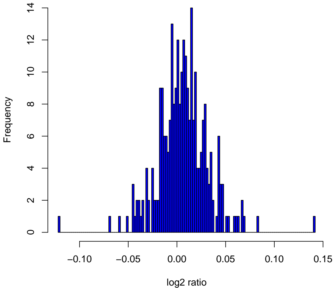
Histogram of log2ratios in 270 HapMap samples at clone Chr11tp-9G1
