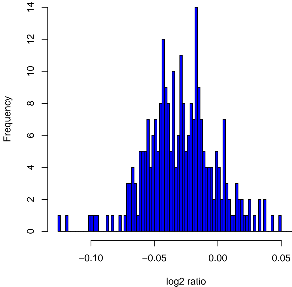
Histogram of log 2 ratios in 270 HapMap samples at clone Chr11tp-9G9
