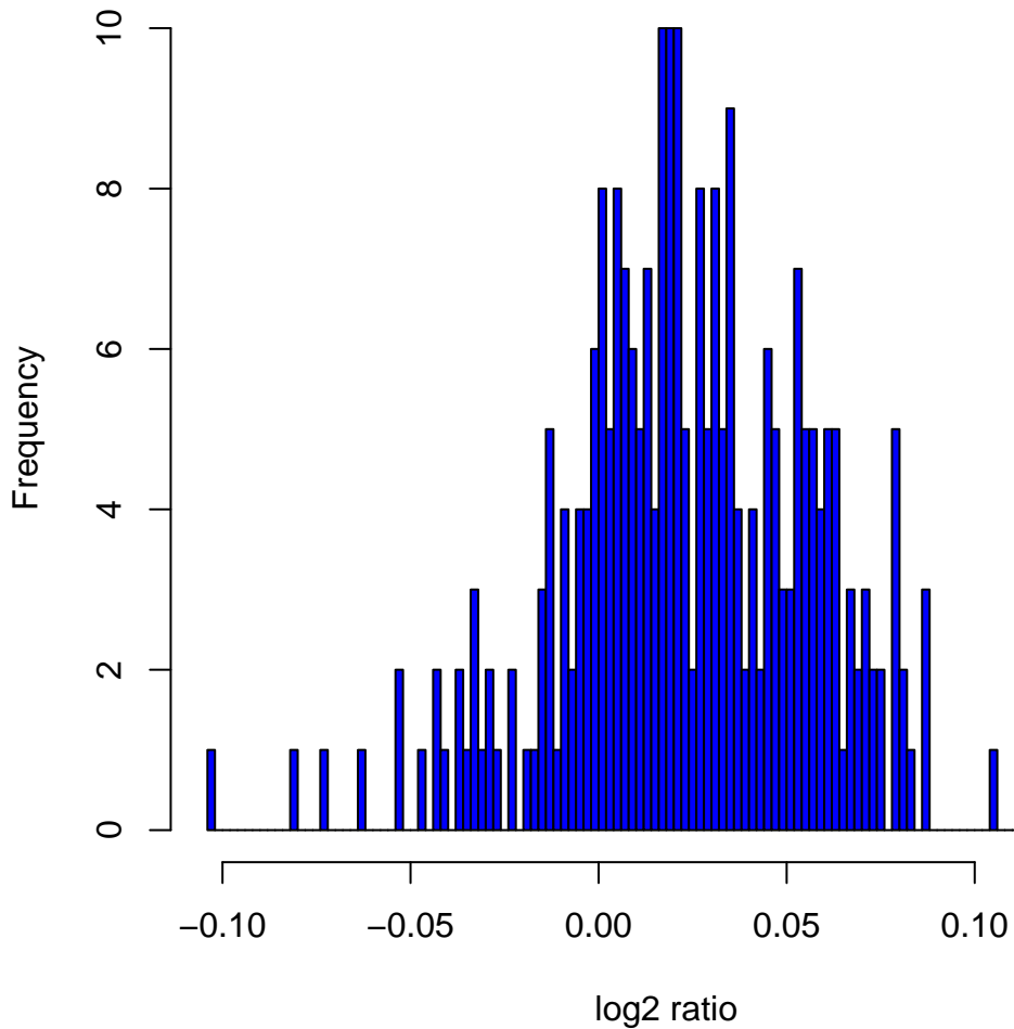
Histogram of log2ratios in 270 HapMap samples at clone Chr12tp-10A5
