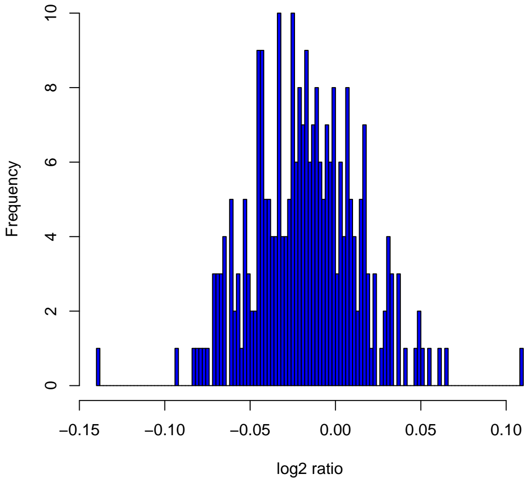
Histogram of log2ratios in 270 HapMap samples at clone Chr12tp-10A7
