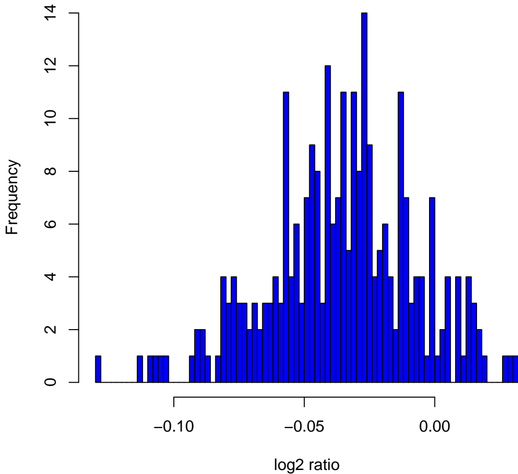
Histogram of log2ratios in 270 HapMap samples at clone Chr12tp-10B7
