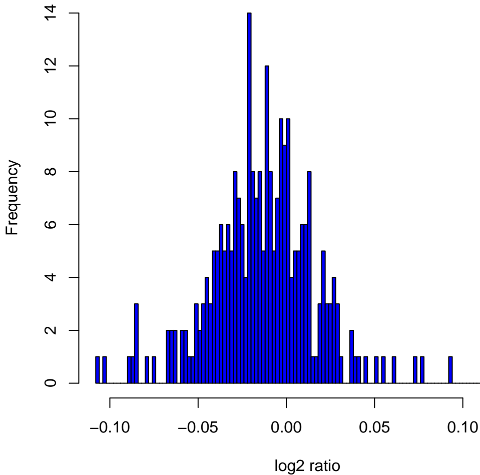
Histogram of log2ratios in 270 HapMap samples at clone Chr12tp-10D2
