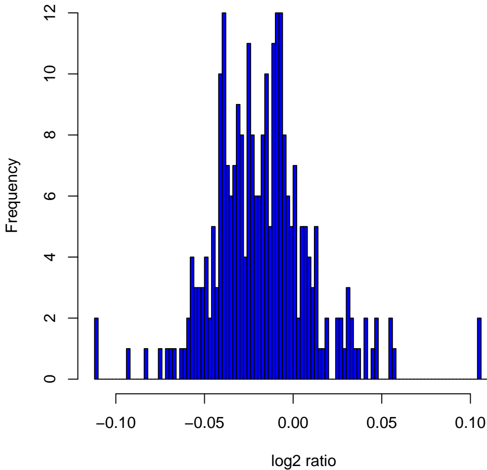
Histogram of log2ratios in 270 HapMap samples at clone Chr12tp-10D6
