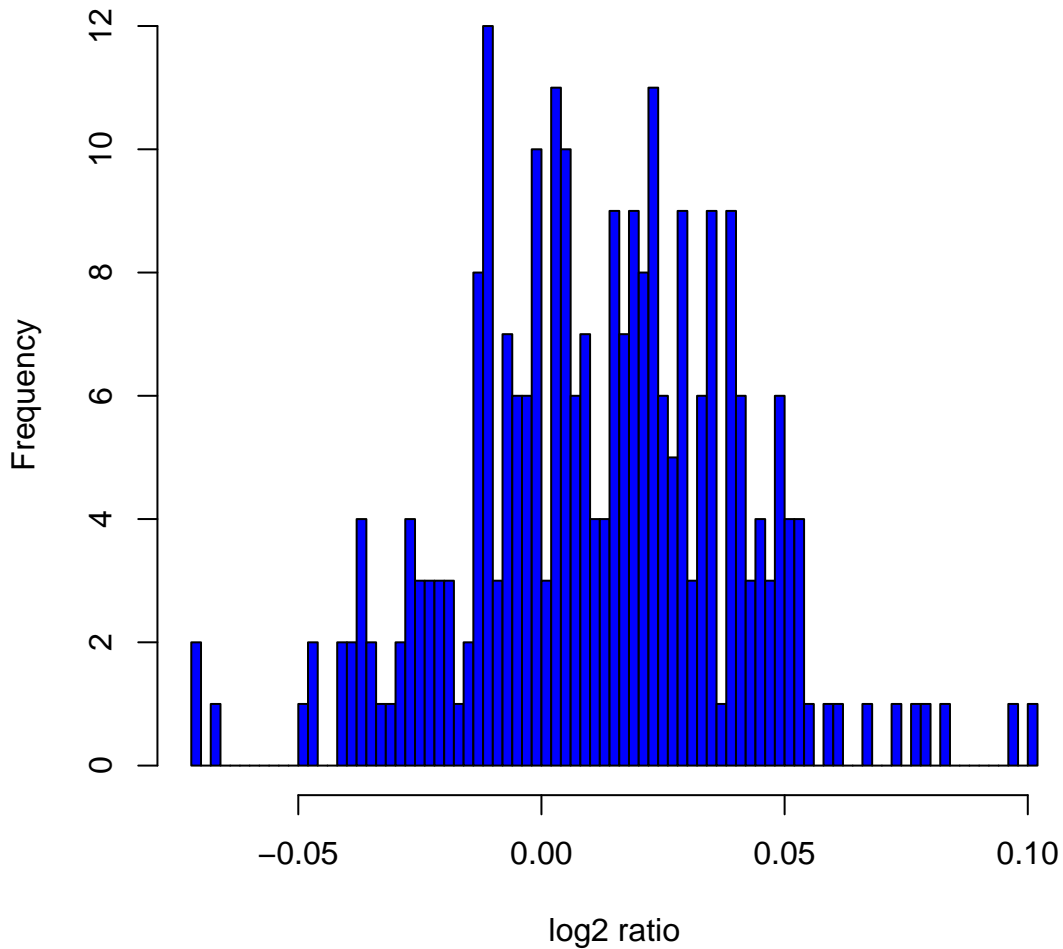
Histogram of log2ratios in 270 HapMap samples at clone Chr12tp-10E4
