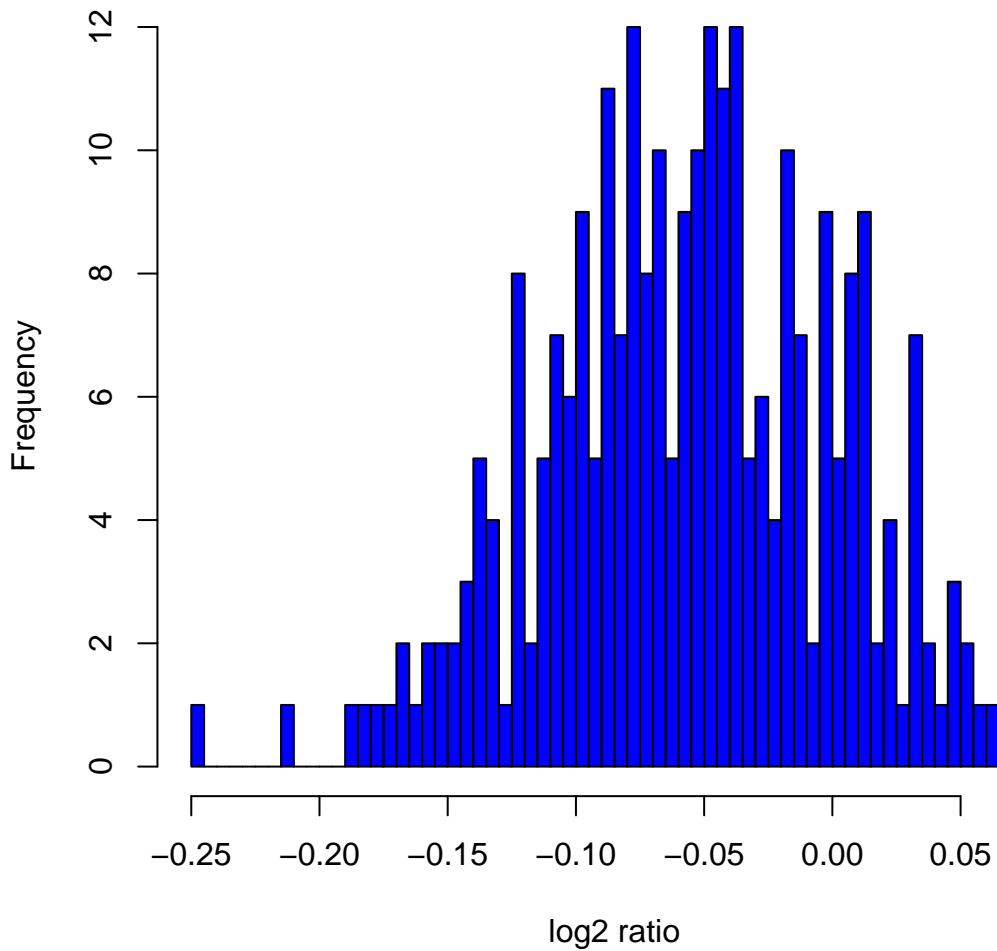
Histogram of log2ratios in 270 HapMap samples at clone Chr12tp-10F12
