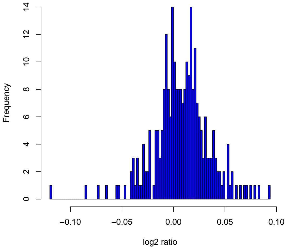
Histogram of log2ratios in 270 HapMap samples at clone Chr12tp-11B10
