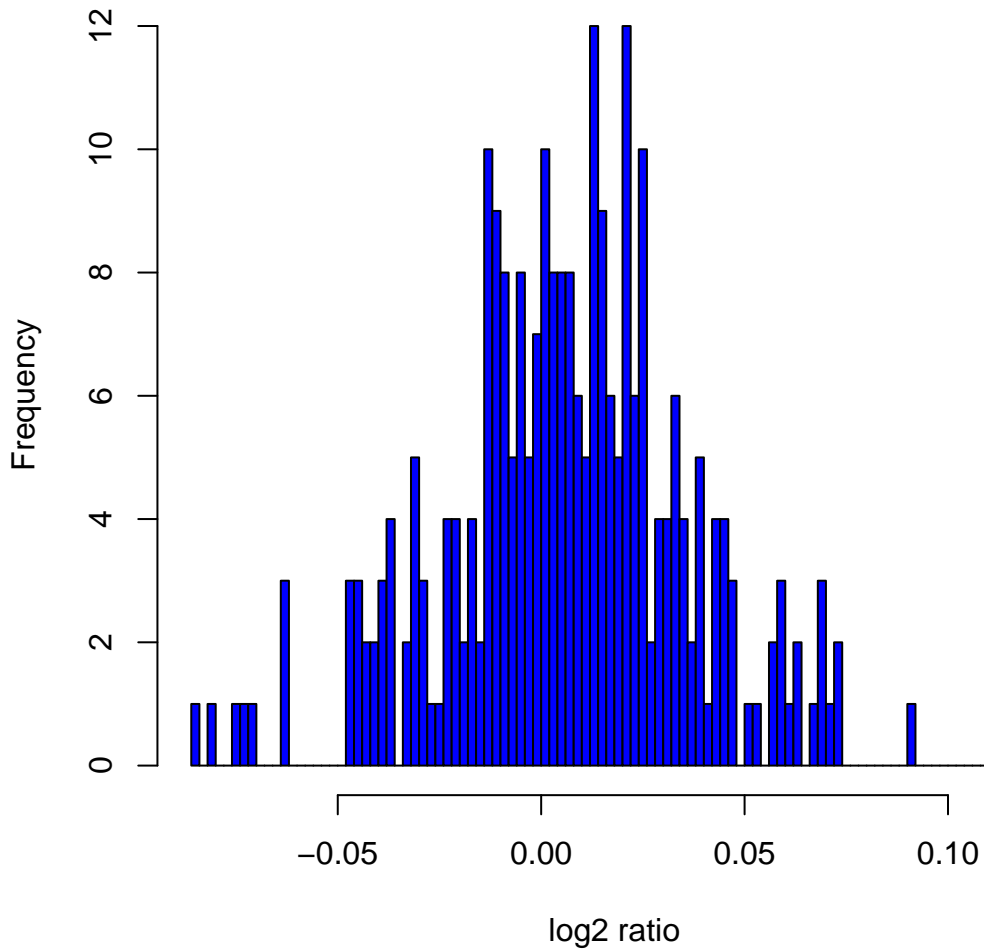
Histogram of log2ratios in 270 HapMap samples at clone Chr12tp-11C2
