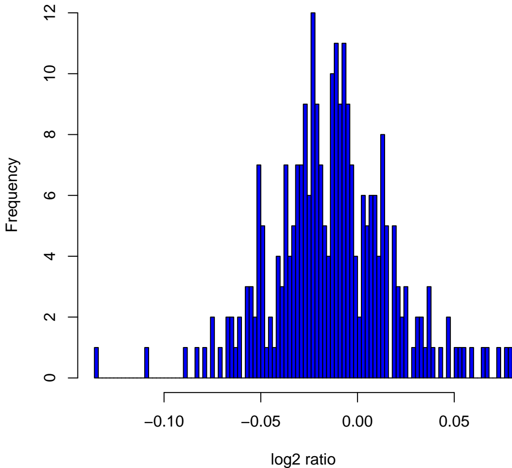
Histogram of log2ratios in 270 HapMap samples at clone Chr12tp-11C3
