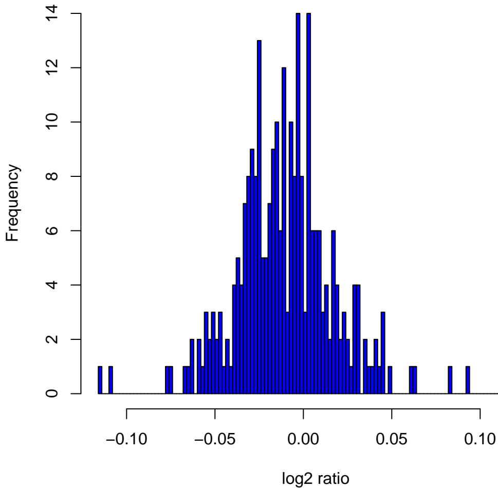
Histogram of log2ratios in 270 HapMap samples at clone Chr12tp-11C8
