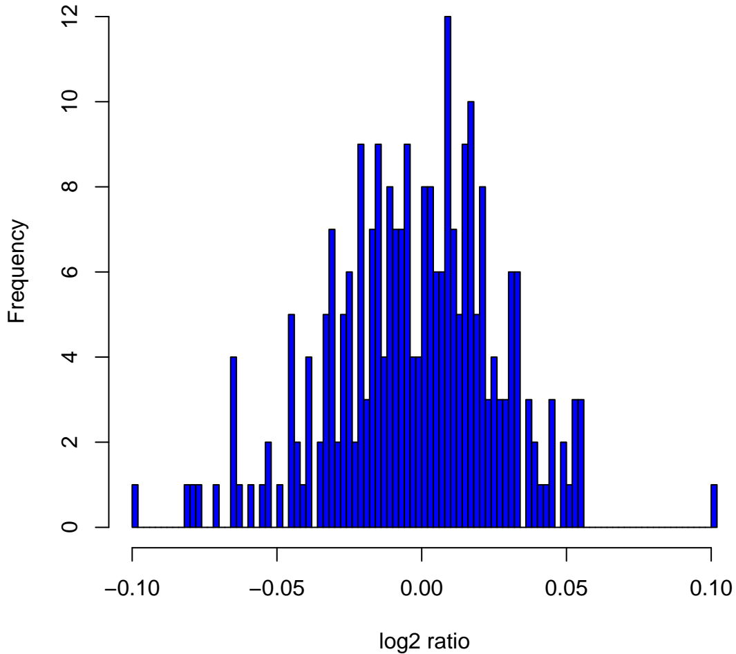
Histogram of log2ratios in 270 HapMap samples at clone Chr12tp-11F5
