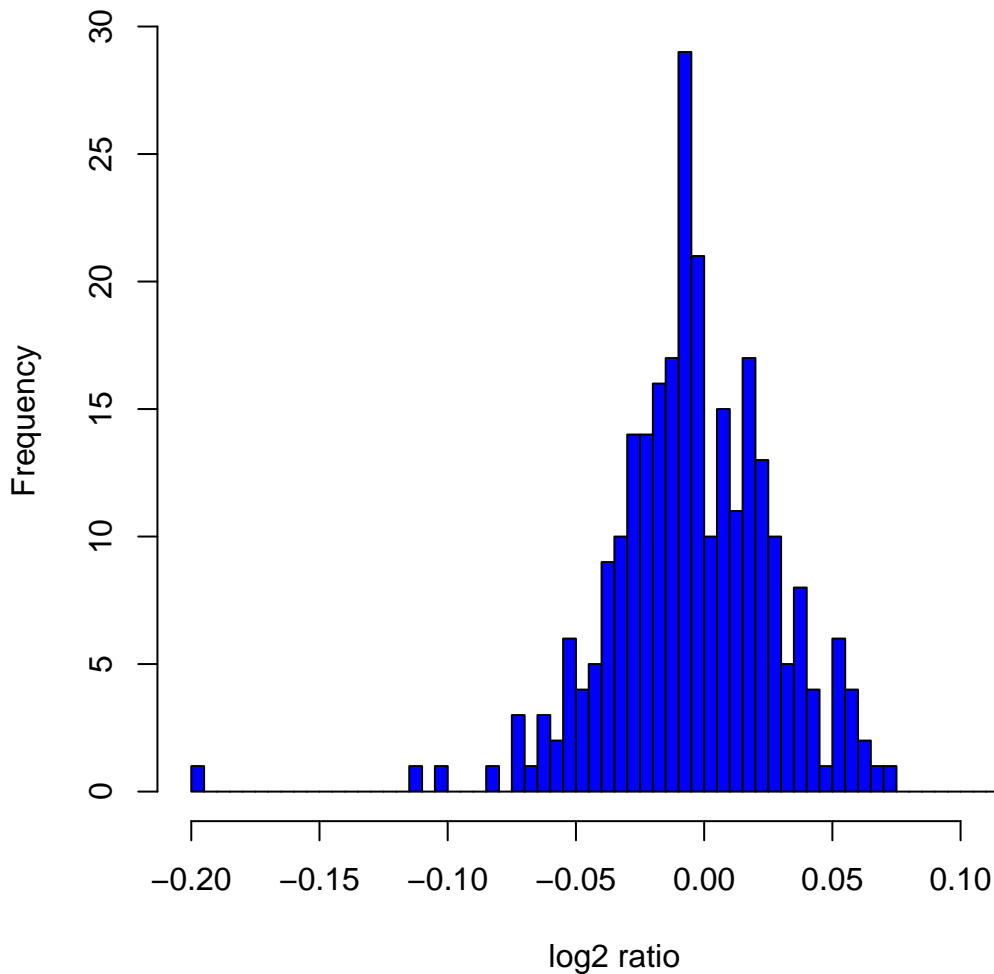
Histogram of log2ratios in 270 HapMap samples at clone Chr12tp-11G1
