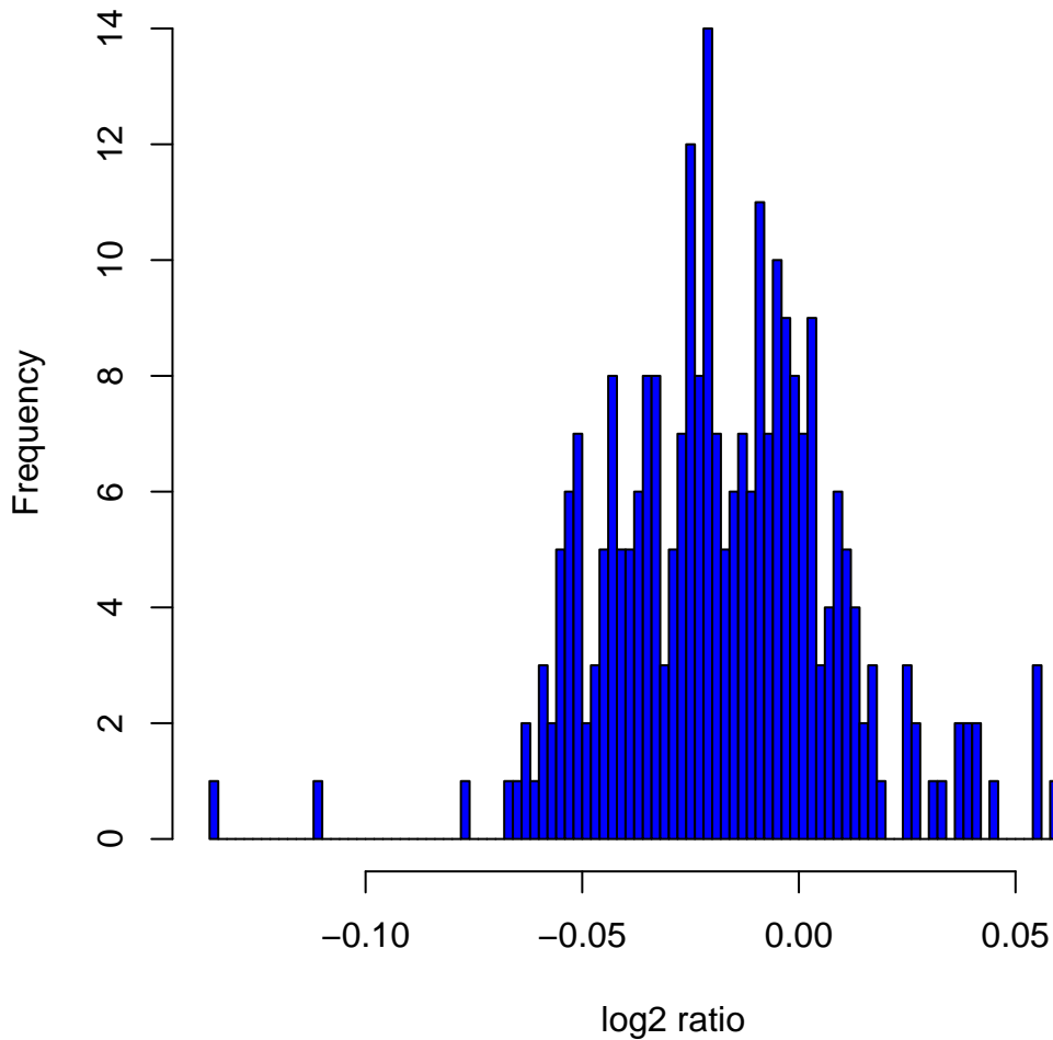
Histogram of \log_2 ratios in 270 HapMap samples at clone Chr12tp-11G2
