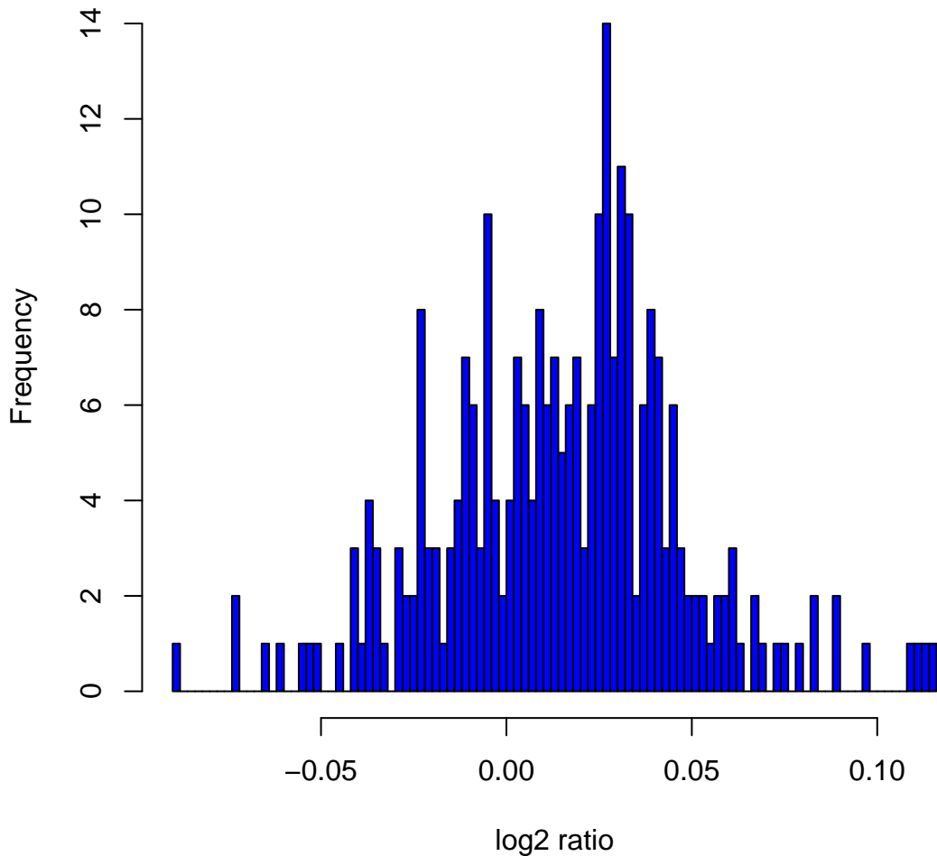
Histogram of log2ratios in 270 HapMap samples at clone Chr12tp-11H6
