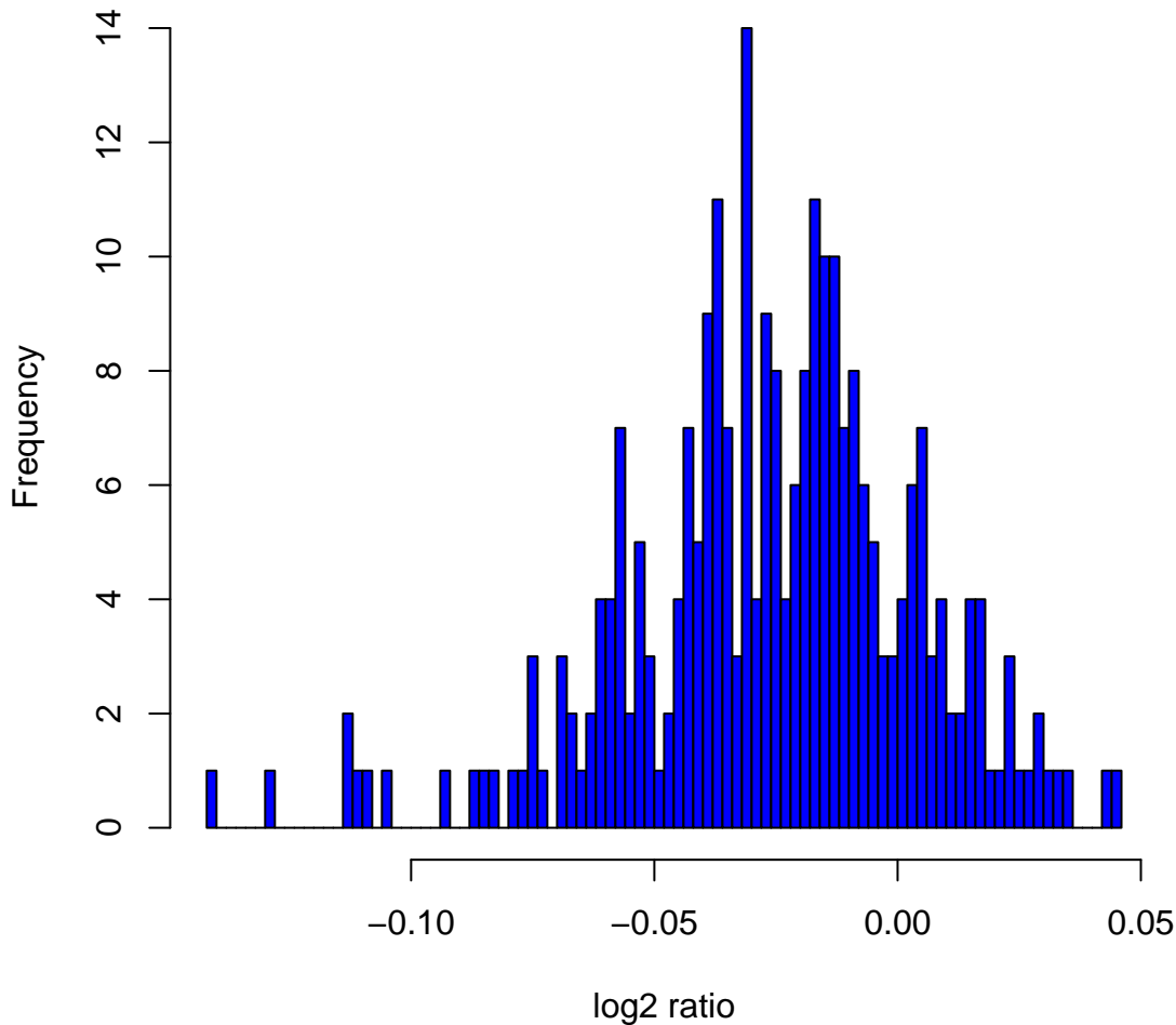
Histogram of log2ratios in 270 HapMap samples at clone Chr12tp-12C2
