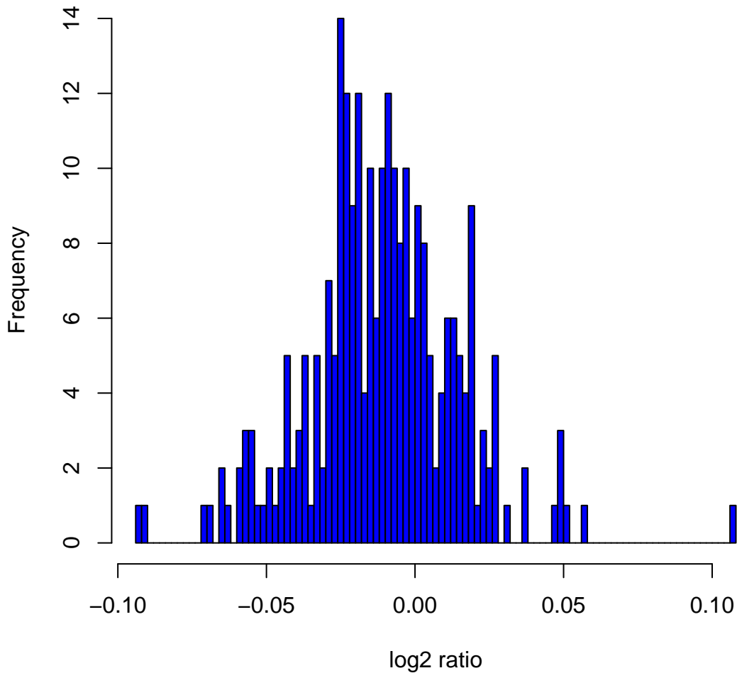
Histogram of log2ratios in 270 HapMap samples at clone Chr12tp-12C8
