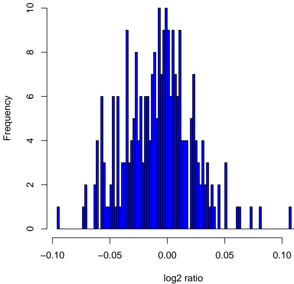
Histogram of log2ratios in 270 HapMap samples at clone Chr12tp-13B12
