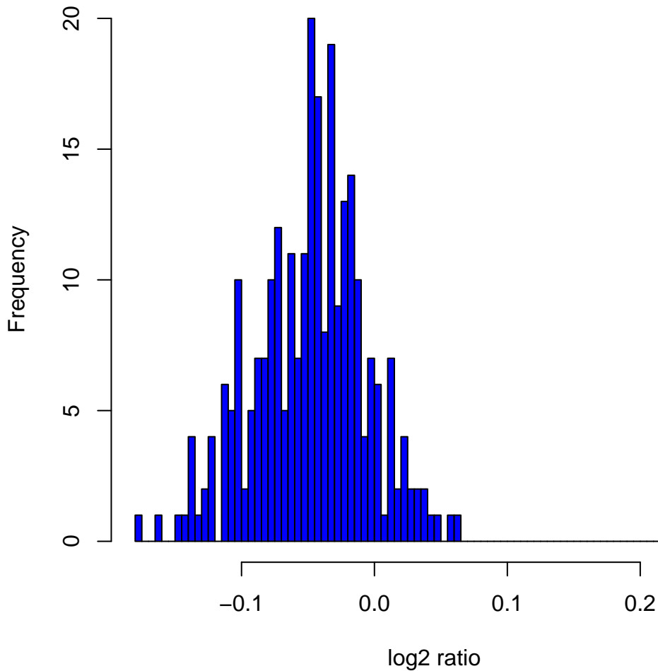
Histogram of log2ratios in 270 HapMap samples at clone Chr12tp-13F8
