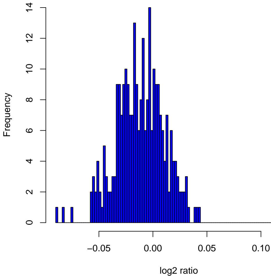
Histogram of log 2 ratios in 270 HapMap samples at clone Chr12tp-16A3
